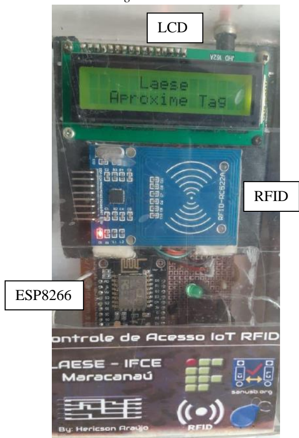
Fig.9: Developed System.
