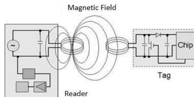
Fig.2: Principle of inductive coupling [26].
