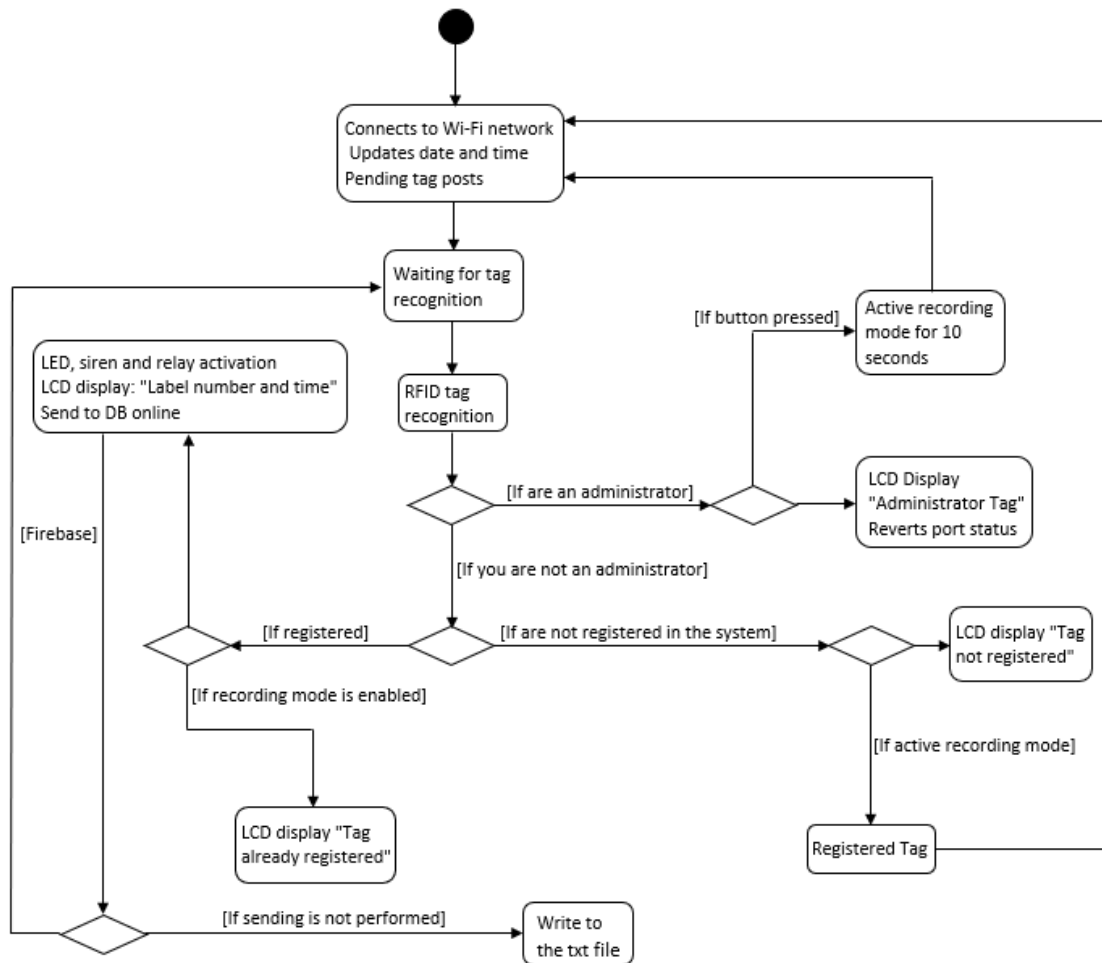
Fig.7: System Flowchart.
