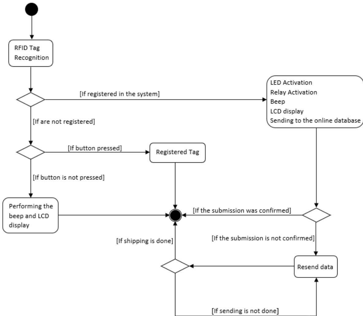
Fig.4: Identification Process Flowchart.
